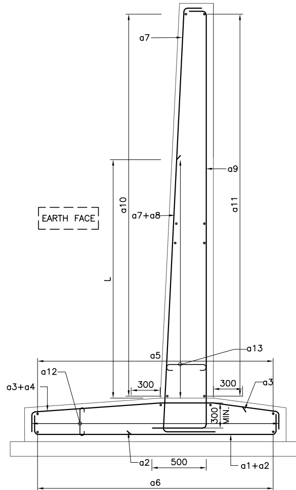
RETAINING WALL SHOWING REINFORCEMENT SCALE-(1:30)
